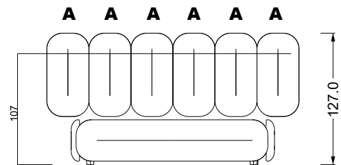
6-er Breite: 243,0 cm
