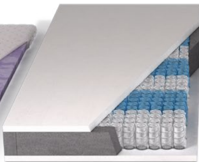
Tonnentaschenfederkernmatratzen Barrel pocket spring core mattresses
