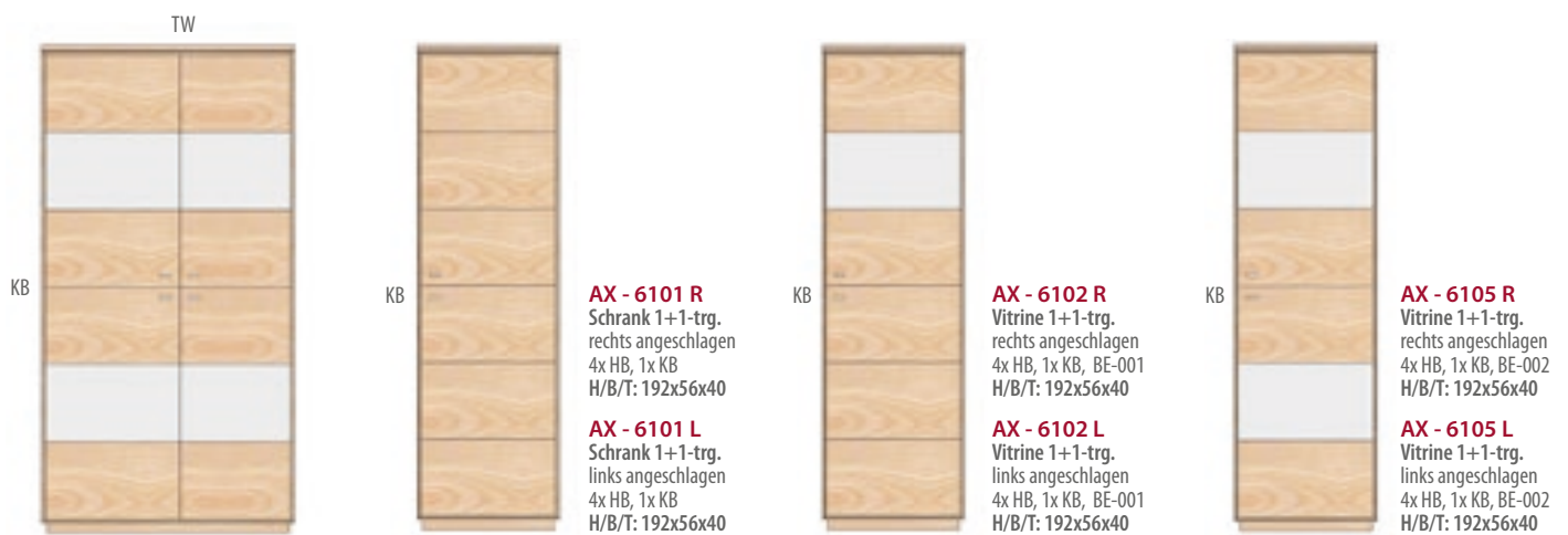
AX - 6201 Schrank 2+2-trg. 8x HB, 2x KB H/B/T: 192x100x40
